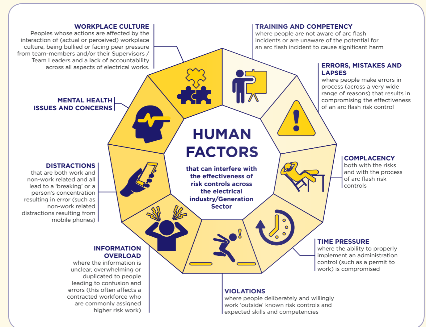
Diagram 5. Human factors
