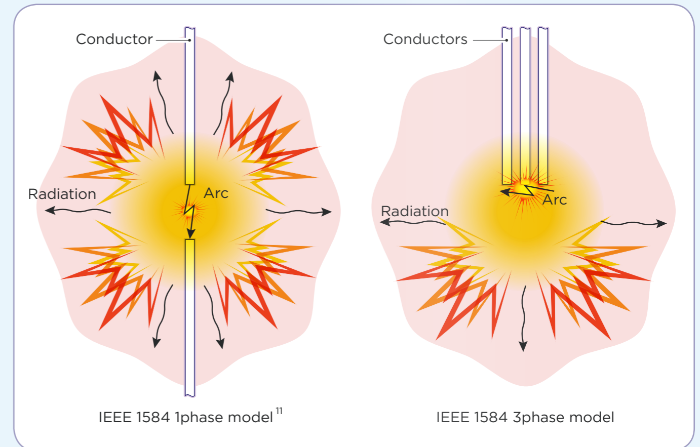
Diagram 23. IEEE 1584 1 and 3 phase models.
