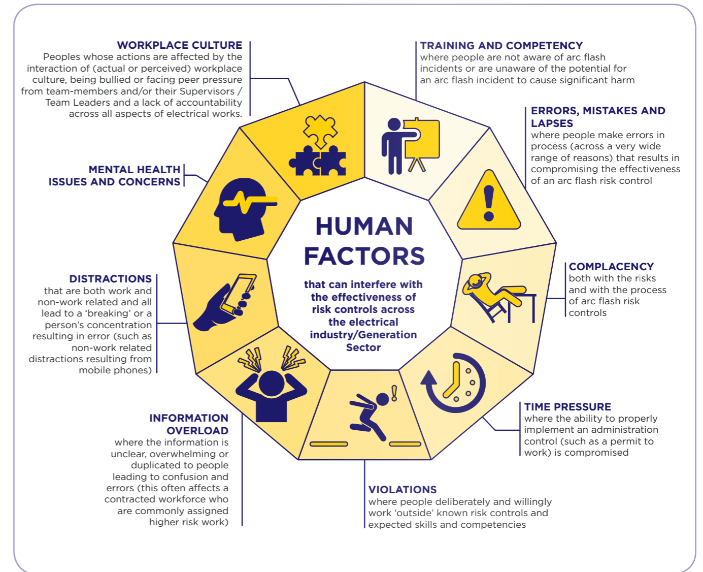
Diagram 14. Human factors
