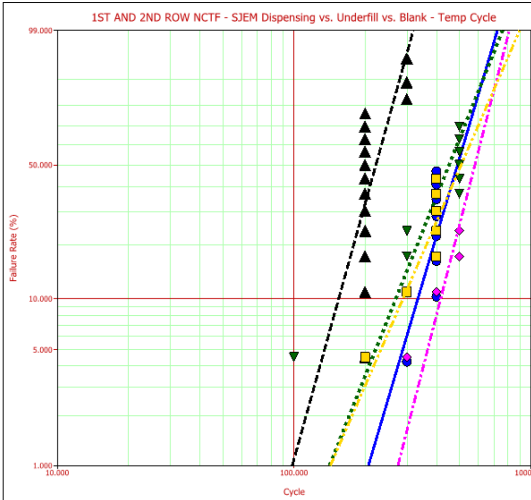
Weibull 2P Maximum Likelihood Plot
