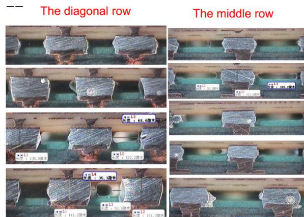
Figure 22. Dis3 material coverage
