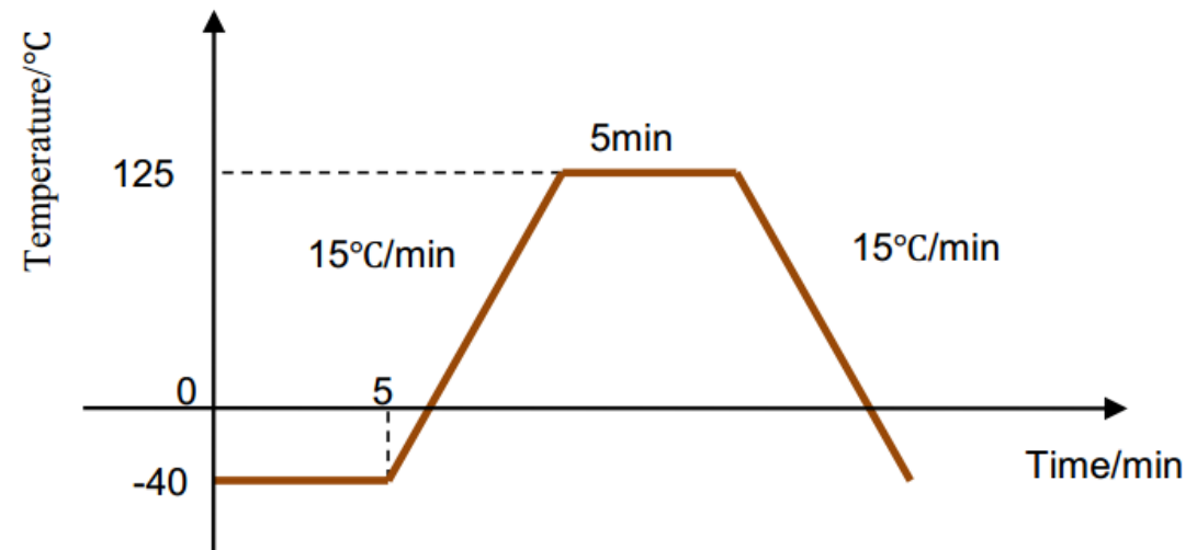
Temperature vs Time Profile
