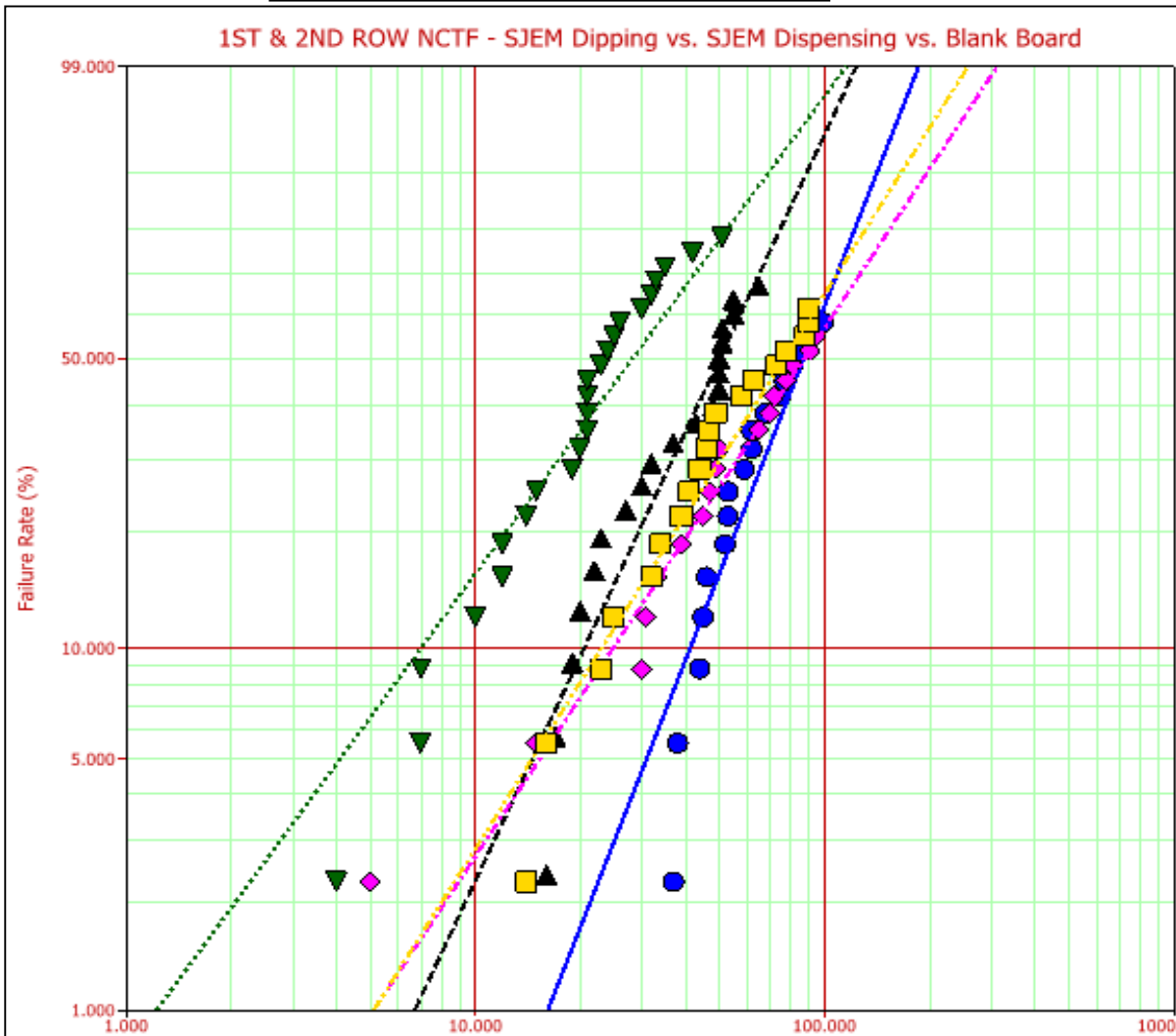
Weibull 2P Maximum Likelihood Plot
