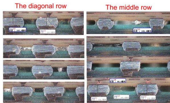
Figure 21. Dis2 material coverage
